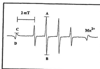
Fig. 12. Typical ESR signal pattern of hydroxyl radicals produced by Fenton's reaction. Relative signal intensity was obtained as the ratio of the distance between A and B, to the distance between C and D.
