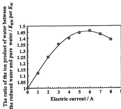
Fig. 7. The ratio ( K_{RW}/K_W ) of the ionic product of reduced water and pure water used as solvent. K_{RW} is the ionic product of water in reduced water, K_W is the ionic product of water in pure water.
