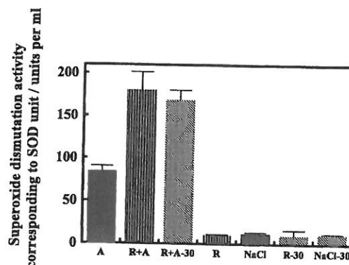
Fig. 10. Superoxide dismutation activity of L-ascorbic acid. A: L-ascorbic acid in 2 mM NaCl solutions, R + A: L-ascorbic acid in reduced water, R + A + 30: L-ascorbic acid in the reduced water 30 days after electrolysis, R: the reduced water, NaCl: 2 mM NaCl solutions, R + 30: reduced water 30 days after preparation and NaCl + 30: 2 mM NaCl solutions 30 days after preparation.
